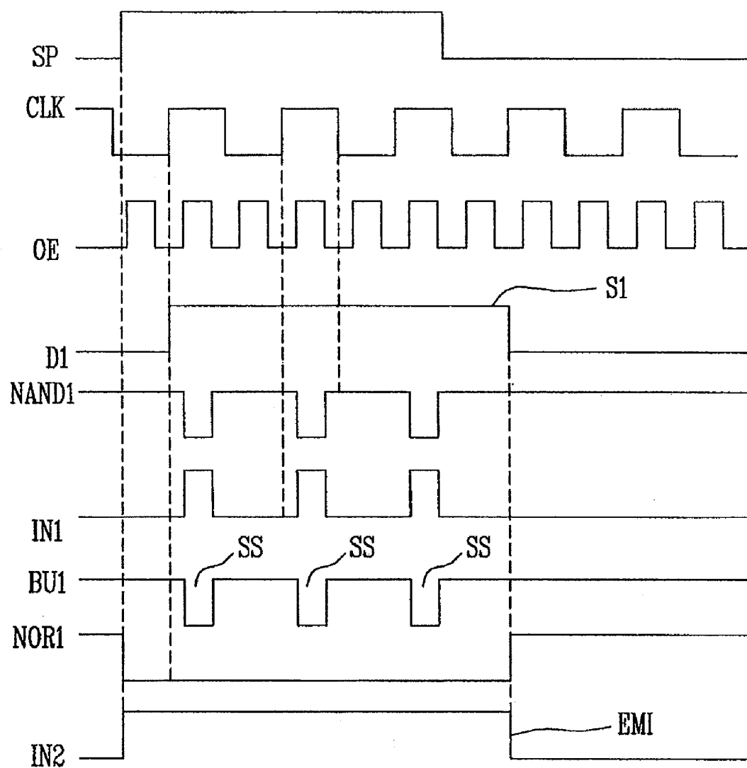
FIG. 3 (PRIOR ART)
